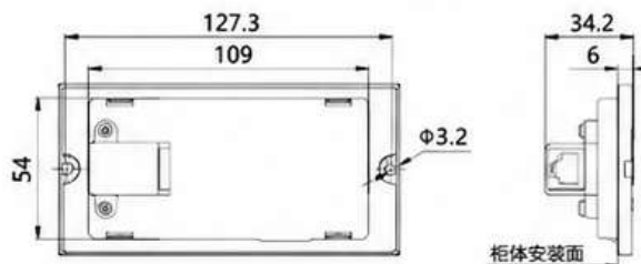
Split liquid crystal screen control module size
