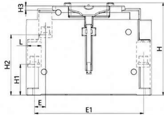
Side view of the integrated type
