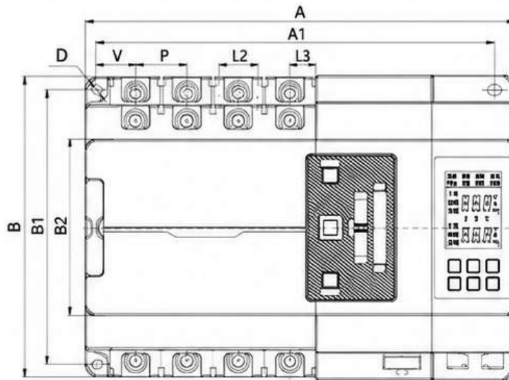
Front view of the integrated type
